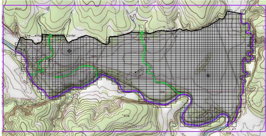
Figure 10 Only active cells are visible
