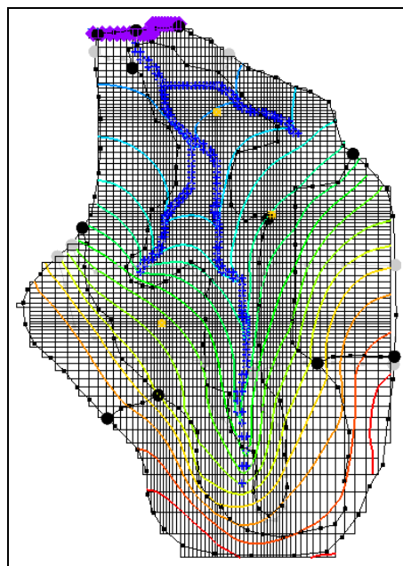
Figure 7 Contours after MODFLOW run
