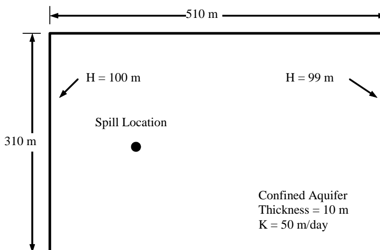
Figure 1 Sample problem to be modeled with RT3D
